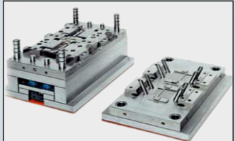
Electric Switch Molud
